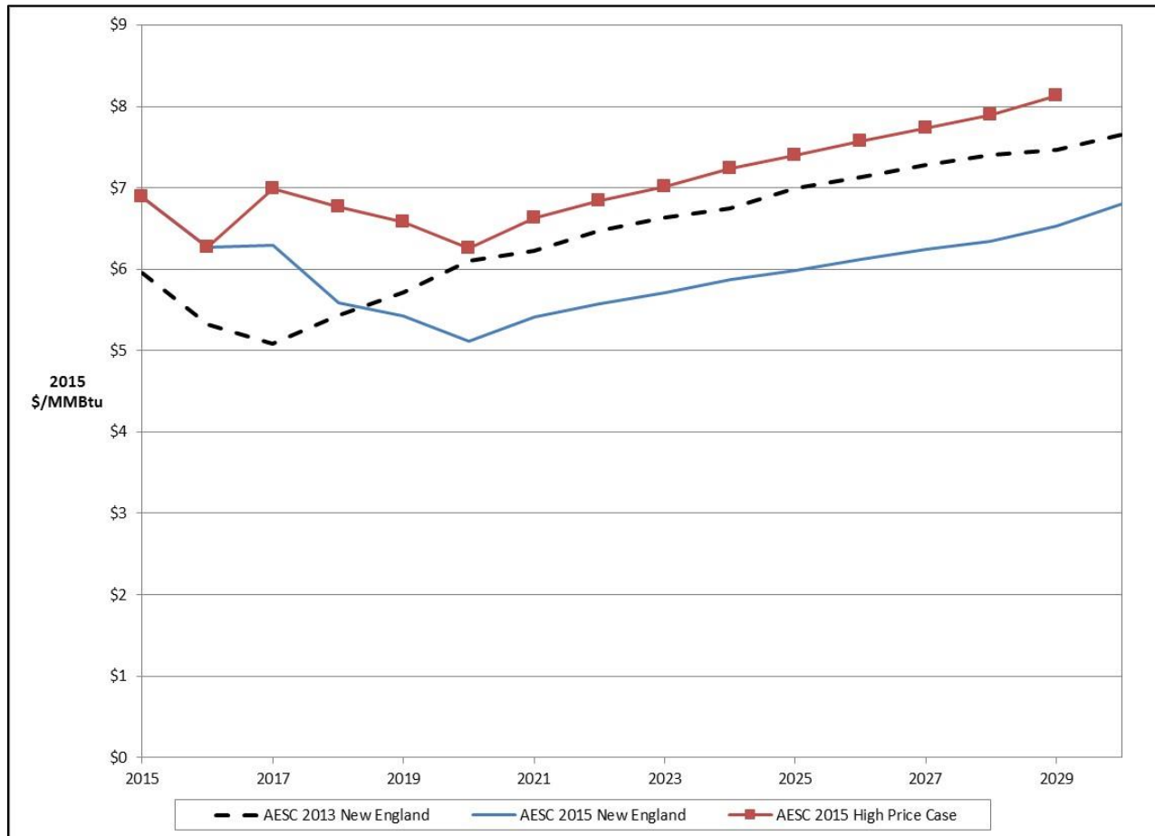
Exhibit 6-18. Annual Wholesale City-Gate Cost of Gas, High Price Case vs. Base Case ($/MMBtu) (2015$)
