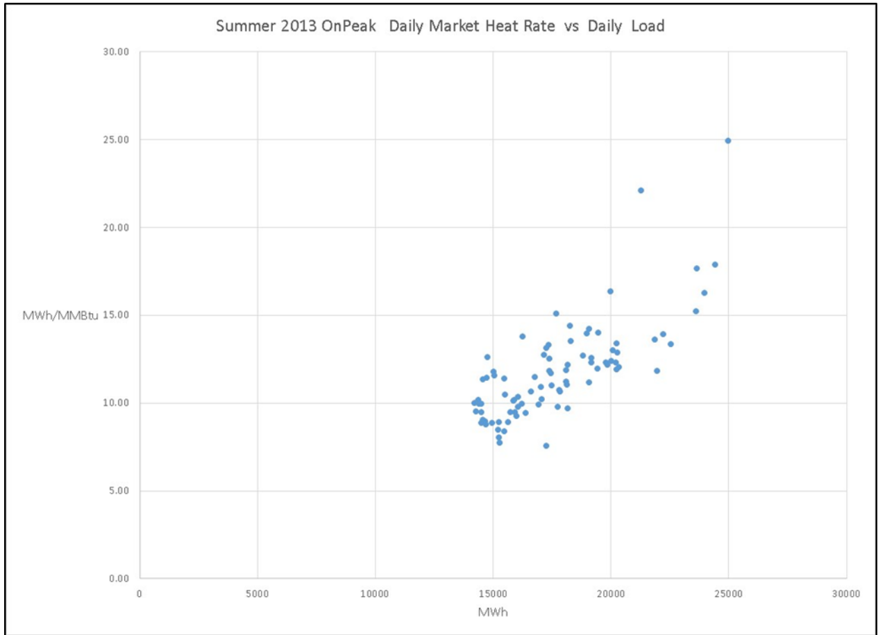
Exhibit 7-6 Summer 2013 On-Peak Daily Market Heat Rate vs Daily Load
